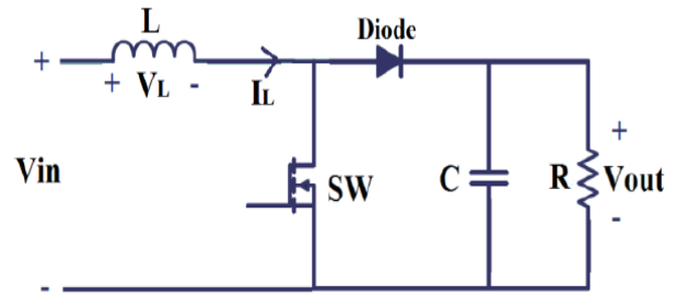
Fig. 6 Electrical circuit of the boost converter
