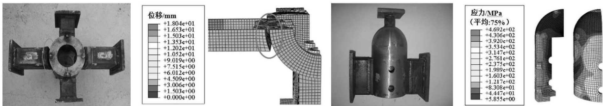
图 6 JD2 试验及数值分析所得的破坏模式 Fig.6 Failure modes of tested specimen JD2 and its FE model
