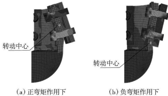
图12 节点最终变形 Fig.12 Final deformation of the joint
