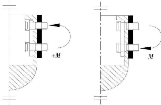
图11 节点受力简图 Fig.11 Force diagram of the joint
