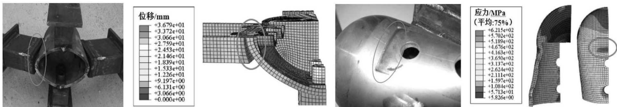
图 5 JD1 试验及数值分析所得的破坏模式 Fig.5 Failure modes of tested specimen JD1 and its FE model
